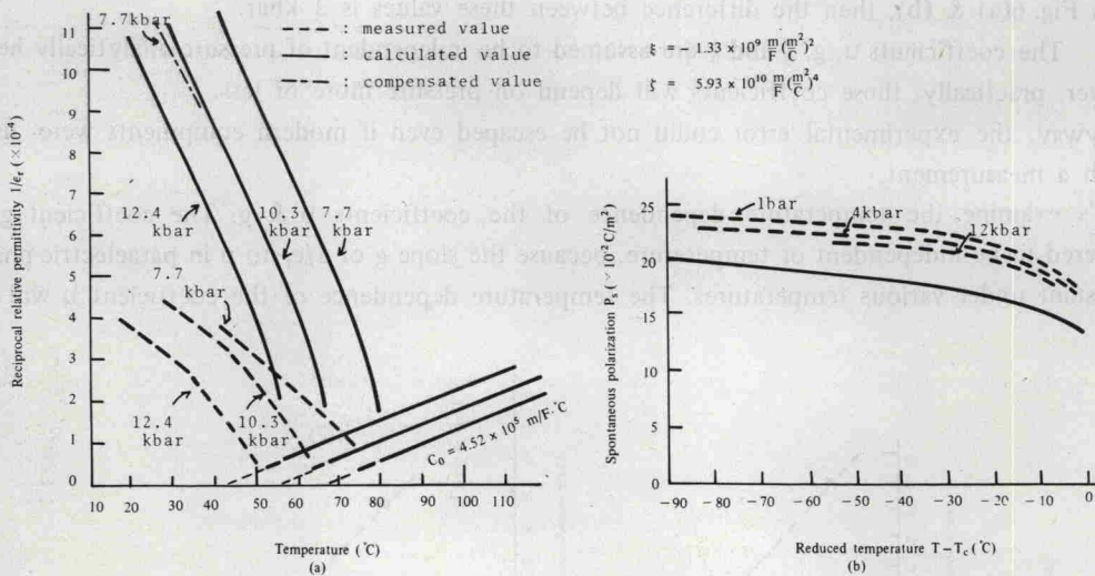
Fig. 8. The temperature dependence of (a) the reciprocal relative permittivity & (b) the spontaneous polarization of single crystal BaTiO 3 with pressure parameter.
